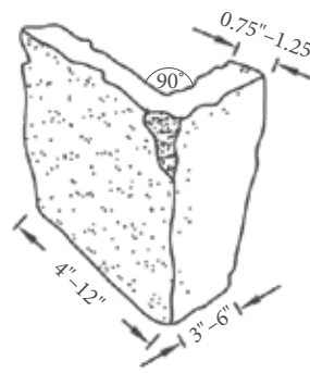
Mosaic/Square Corner
