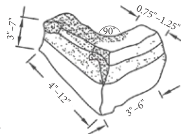
Ashlar Corner
